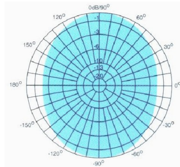
Horizontal Plane
